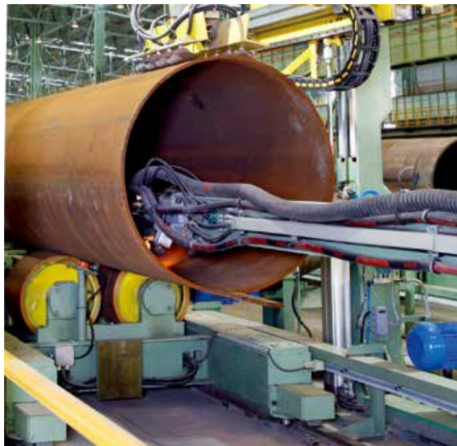
Internal welding
